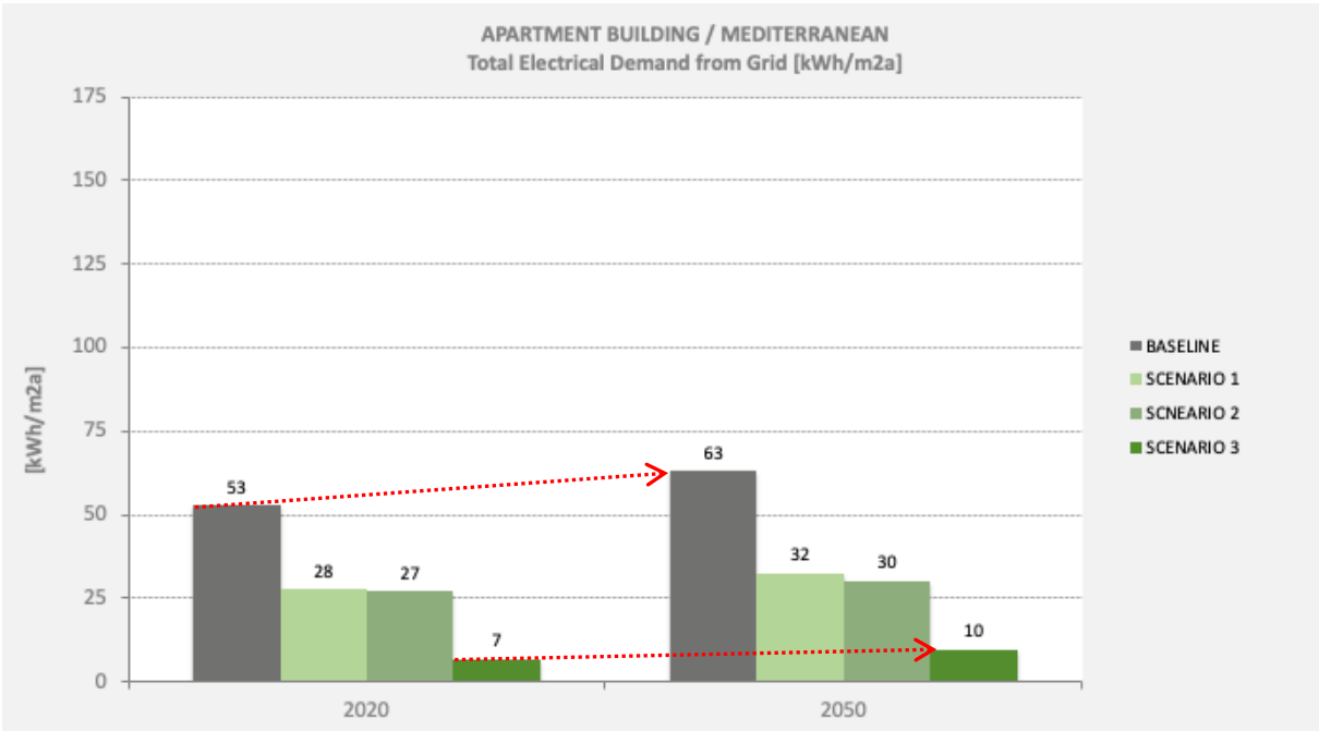
Figure 7: Impacts of climate change by 2050 on electrical energy demand, example apartment building in mediterranean climate zone (Source: Österreicher, Seerig (2020), Building Climate Study)
