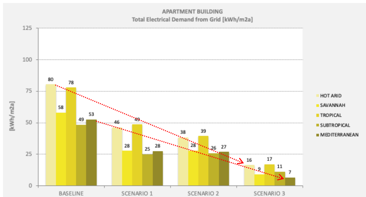
Figure 5: Electrical energy reduction potential per improvement scenario, example apartment building (Source: Österreicher, Seerig (2020), Building Climate Study)
