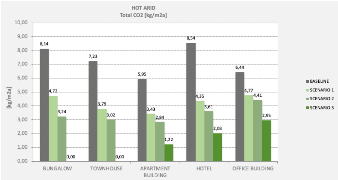
Figure 4: CO 2 reduction potential per building type, highlighting bungalow and hotel types (Source: Österreicher, Seerig (2020): Building Climate Study)
